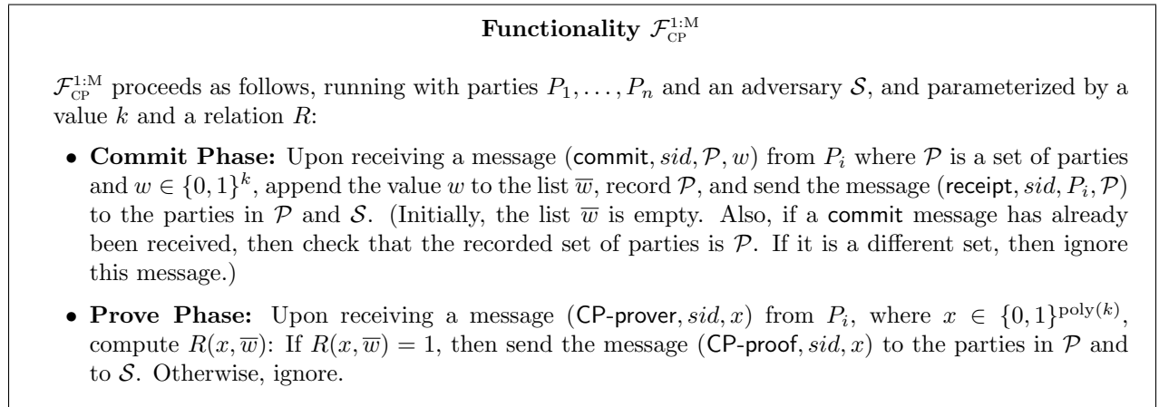
Figure 15: One-to-Many commit-and-prove
