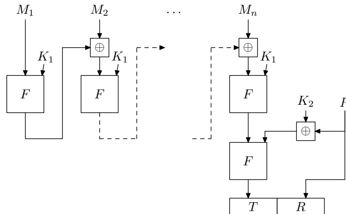
Fig. 1. The RMAC tagging algorithm with keys K_1, K_2 on input M_1 \parallel M_2 \parallel \dots \parallel M_n . The underlying block cipher is denoted F . The randomness R is chosen anew on each invocation. The resulting tag is T \parallel R .
