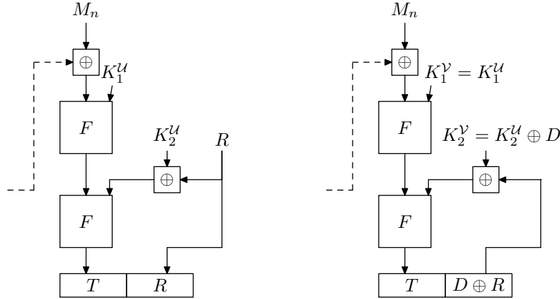
Fig. 2. The RMAC known-difference related-key attack (Section 5). The figure on the left shows how user \mathcal{U} constructs a tag (T, R) for a message M in response to an adversary's query. The figure on the right suggests why user \mathcal{V} will accept (T, D \oplus R) as a tag for message M .
