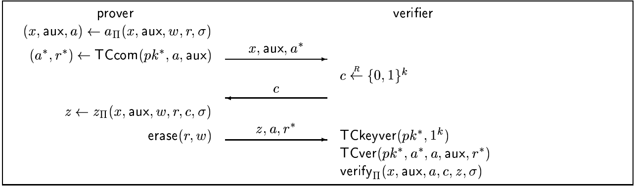
Figure 5: \text{UC}_{[pk^*, vk, \sigma']}^R(x; \text{aux}) : A UCZK protocol for R with common reference string (pk^*, vk, \sigma') drawn from \mathcal{D}_{pk}(\text{TC}) \times \mathcal{D}_{vk}(\text{SIG}_0) \times \mathcal{D}_{\sigma}(\Omega^R) , common input x , and auxiliary input \text{aux} where \Pi = \text{NM}_{[vk, \sigma']}^R(x; \text{aux}) :
