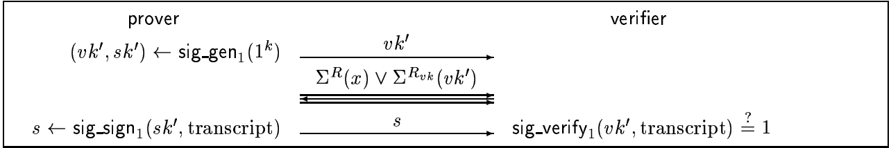
Figure 1: \text{USS}_{[vk]}^R(x) : An unbounded simulation-sound ZK protocol for relationship R with CRS vk (drawn from the distribution \text{sig\_gen}_0(1^k) ), and common input x . The prover also knows the witness w such that R(x, w) = 1 .
