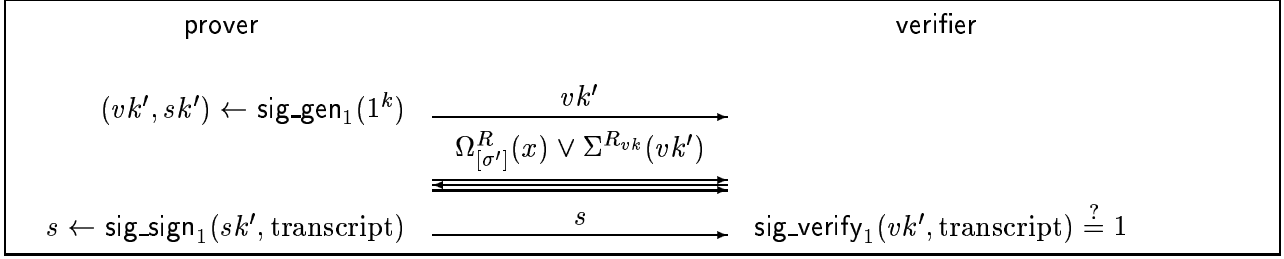
Figure 2: \text{NM}_{[vk, \sigma']}^R(x) : A non-malleable ZK protocol for relationship R with common reference string (vk, \sigma') where \sigma' is drawn from the distribution associated with \Omega_{\sigma'}^R , and common input x .
