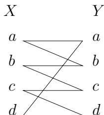
Figure 7: The distribution arising from the “noisy-typewriter channel.”
