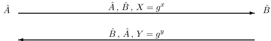
Figure 1: The basic (unauthenticated) Diffie-Hellman protocol
