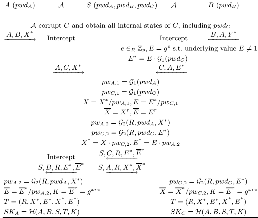
Fig. 14. Execution of 3PAKE in the presence of a malicious adversary
