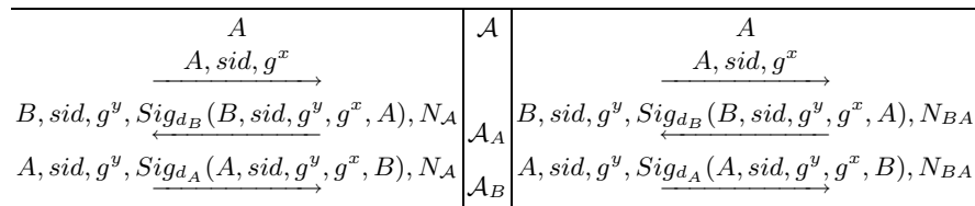
Fig. 12. Execution of the modified (Canetti–Krawczyk) Diffie–Hellman protocol in the presence of a malicious adversary
