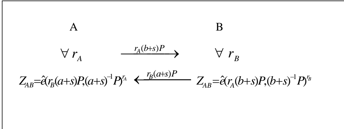
Figure 3: McCullagh-Barreto's Protocol
