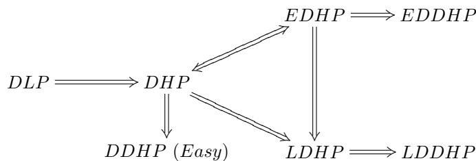
Figure 1: Problem Hierarchy
