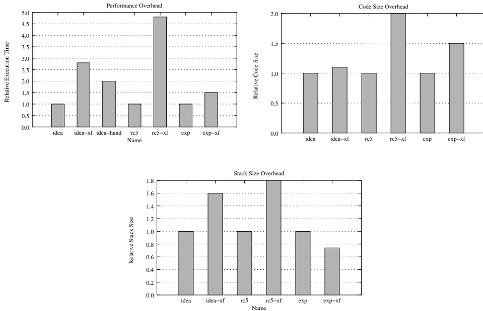
Figure 9: The speed, code size, and stack size overhead of our transform, as applied to modular exponentiation, IDEA, and RC5. The -xf suffix indicates the automatic application of our transform, while the -hand suffix indicates a hand-optimized application of our transform. Values are normalized: the untransformed version of a program takes unit time by definition, while the transformed version of the same program is shown with the relative multiplicative overhead compared to the untransformed version.
