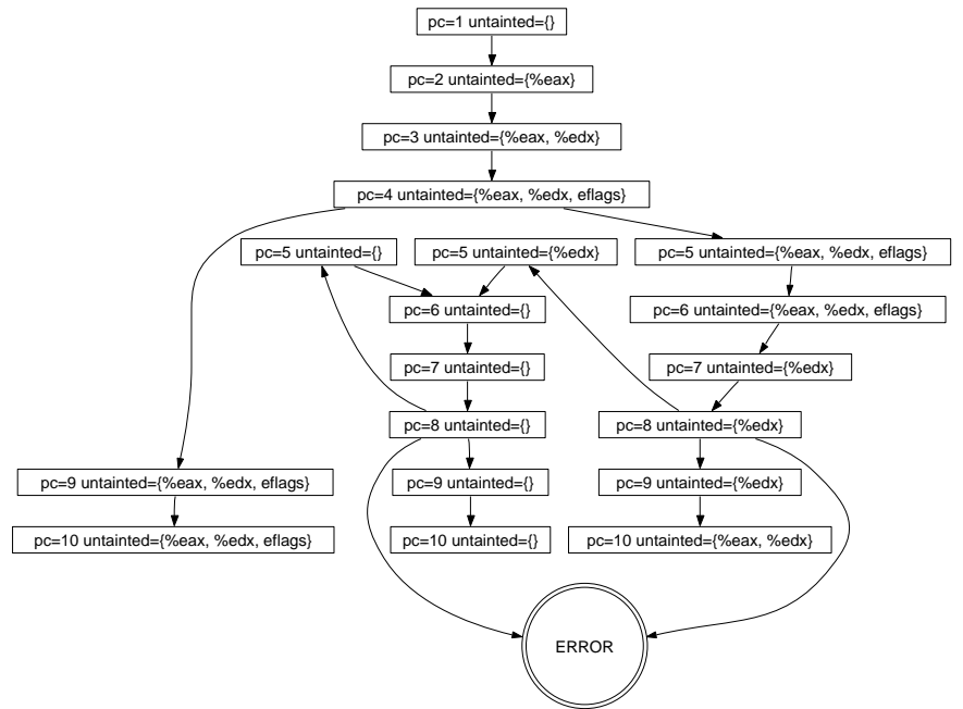
Figure 10: Example: State space explored by the static verifier.
