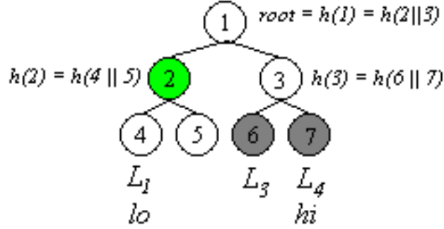
Figure 1: An example CRT query for node L_3 .
