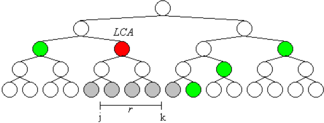
Figure 2: The LCA and co-path nodes for a given (j, k) range.
