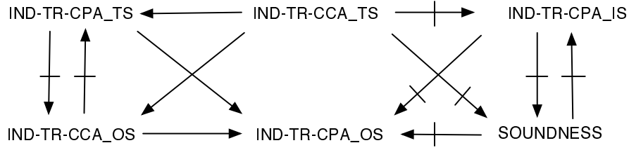
Figure 1: Relations among the security notions
