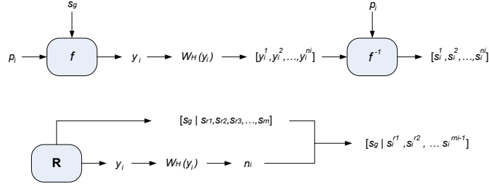
Fig. 5: Multiple leakages experiments: real S-boxes and random S-boxes simulation.
