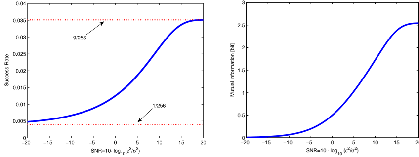
Fig. 3: Success rate and mutual information in function of the SNR.
