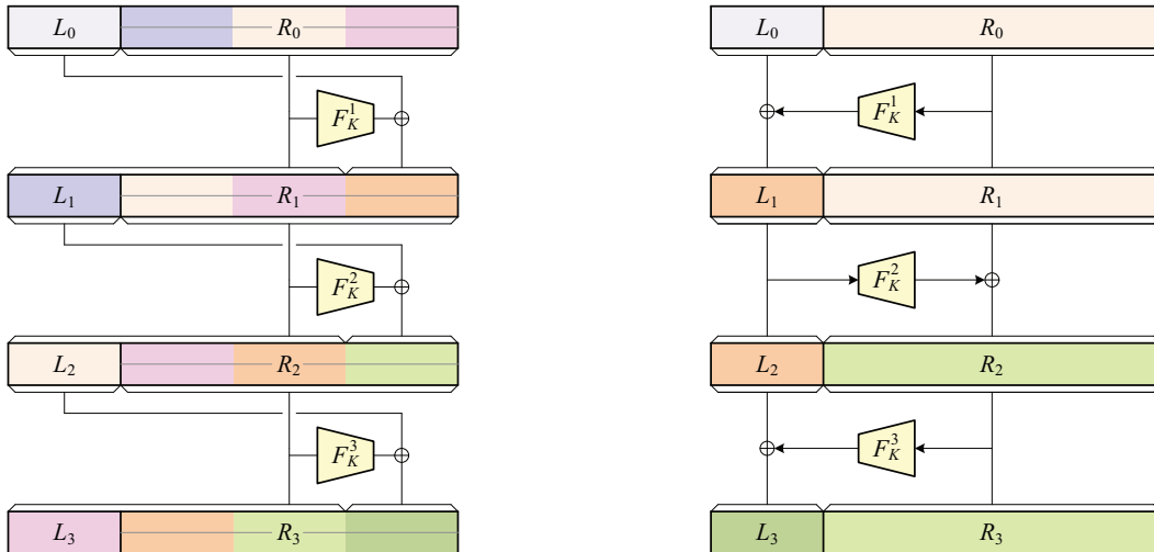
Fig. 4. Diagrams of three rounds of FE1 (left) and FE2 (right) for format N = (a, b) = (2^{n_0}, 2^{n_1}) and input X \in \mathbb{Z}_{ab} . For both mechanisms, L_0, L_1, L_2, L_3 \in \mathbb{Z}_a and R_0, R_1, R_2, R_3 \in \mathbb{Z}_b .
