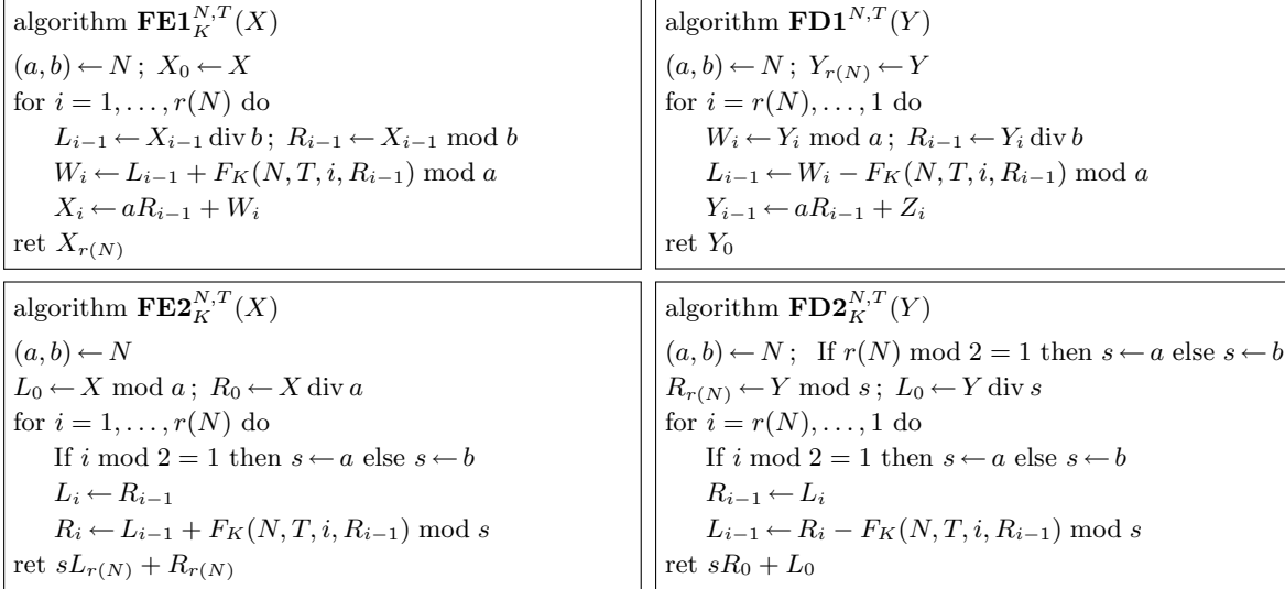
Fig. 3. Top: Encryption and decryption algorithms for the integer FPE scheme FE1 where K \in \mathcal{K} , T \in \mathcal{T} , F \in \mathcal{N} , and X, Y \in \mathcal{X}_F . Here x \text{ div } y is short-hand for \lfloor x/y \rfloor . Bottom: Encryption and decryption algorithms for the integer FPE scheme FE2.
