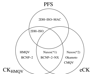
Fig. 1. Security of two-message protocols
