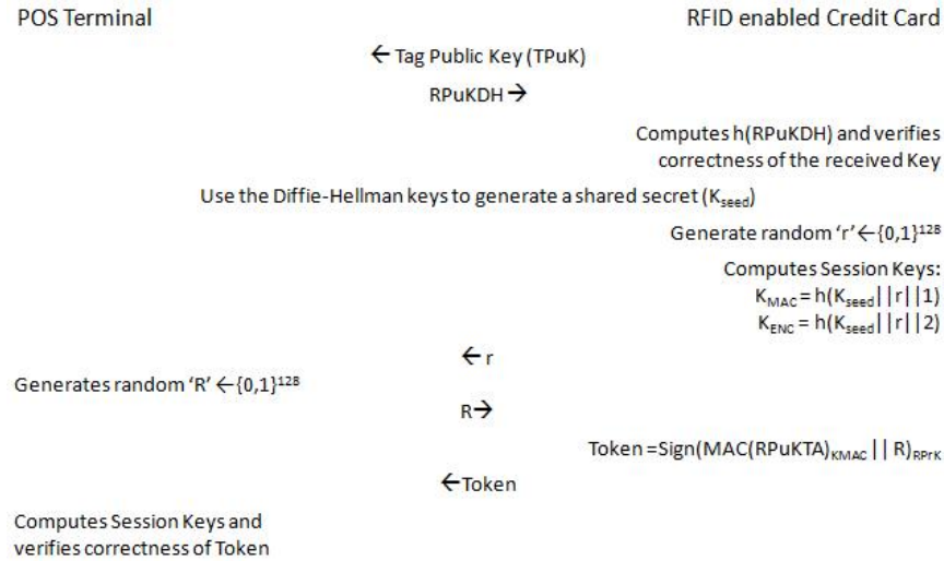
Fig. 11. Tag Authentication
