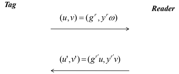
Figure 3: Readers re-encrypt ciphertexts received from tags
