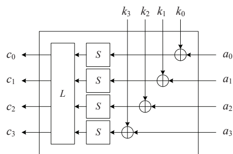
Fig. 2. The round function F of SMS4
