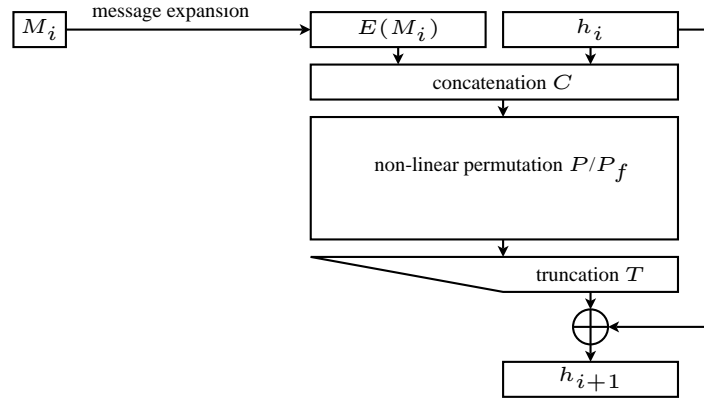
Fig. 1. Domain extension algorithm of Hamsi.
