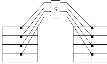
Fig. 4. 4×4 Sbox is used in a bitsliced way in the substitution layer.
