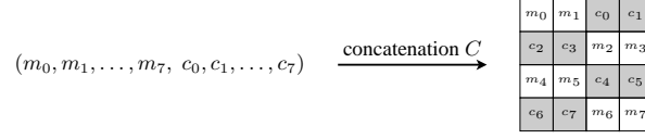
Fig. 2. Concatenation of expanded message words m_0, \dots, m_7 and chaining value words c_0, \dots, c_7 in Hamsi.
