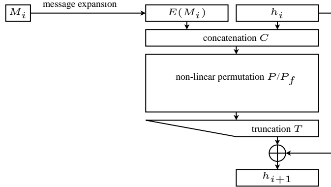
Fig. 1. Domain extension algorithm of Hamsi.
