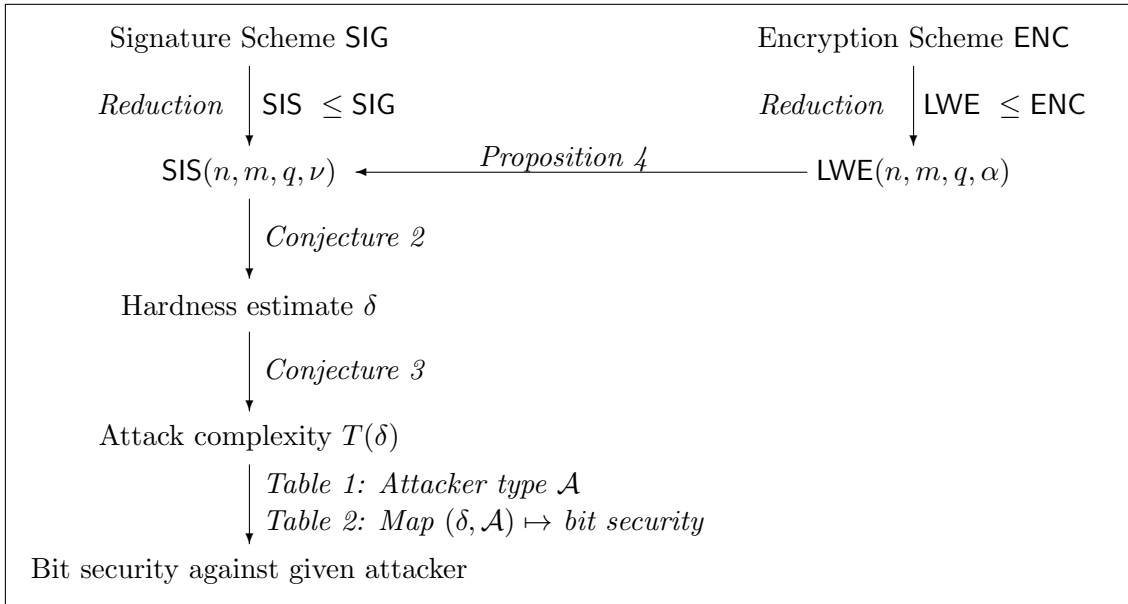
Figure 1: User’s guide to estimating the bit security of lattice-based signature and encryption schemes.
