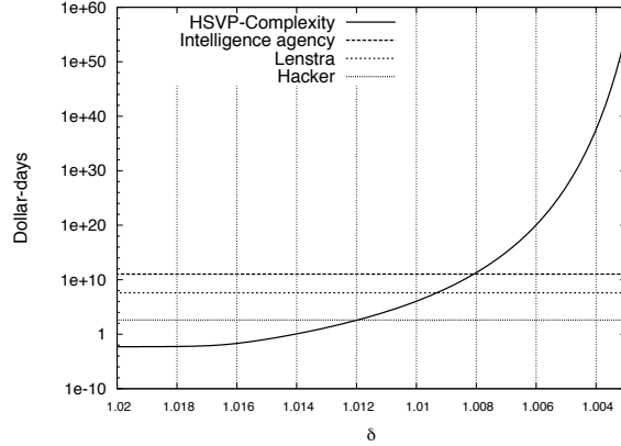
Figure 3: Estimated time complexity of \delta -HSVP for \delta \in [1.003, 1.02] . The plots include horizontal lines, illustrating today’s power of different attacker types.
