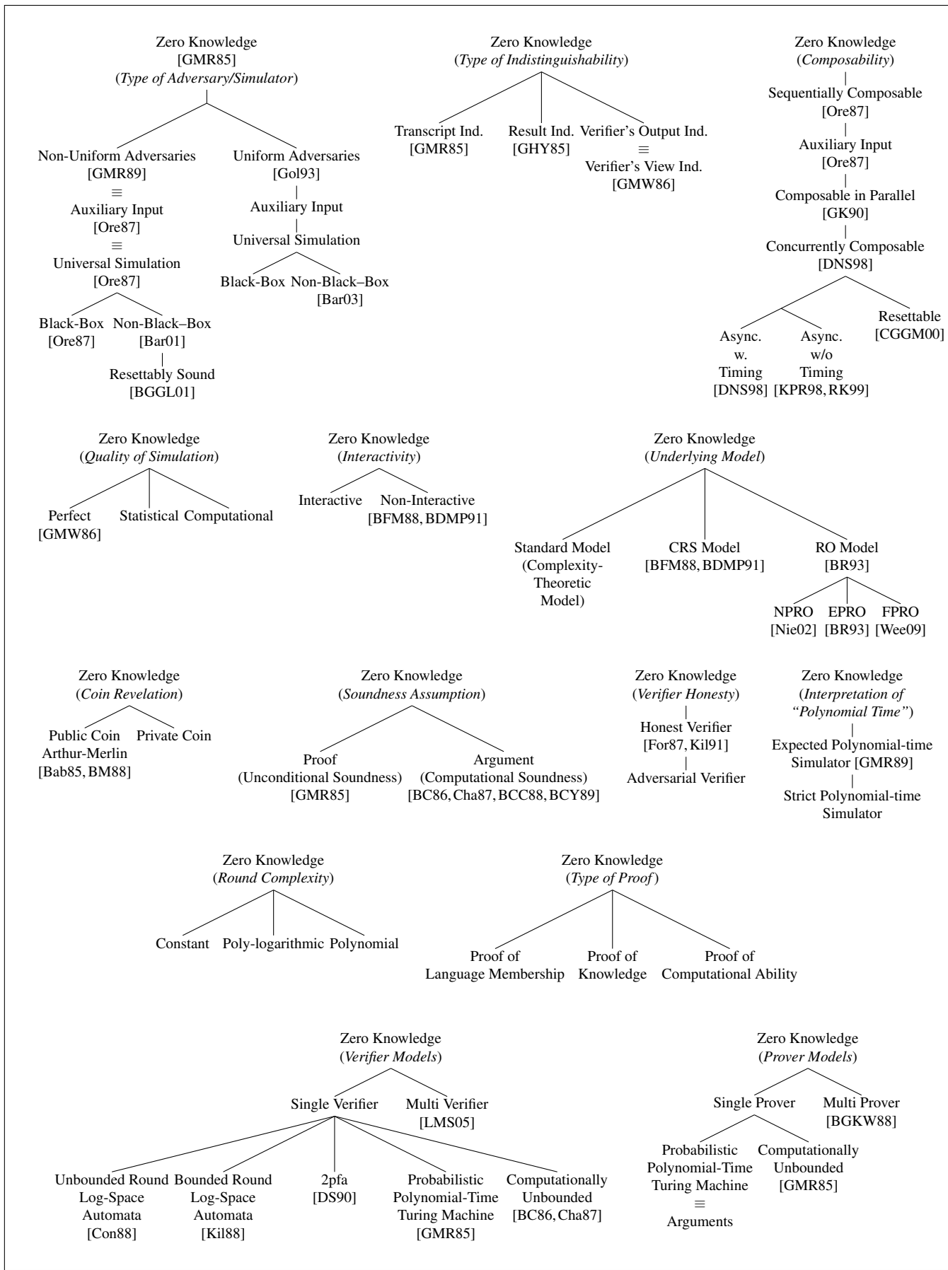
Fig. 1. Several Hierarchies of Definitions of Zero Knowledge
