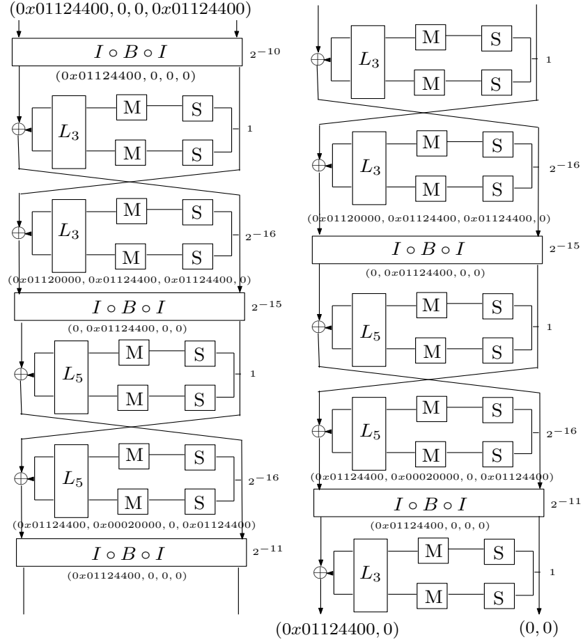
Fig. 3. A 4.75-round differential characteristic with probability 2^{-126}
