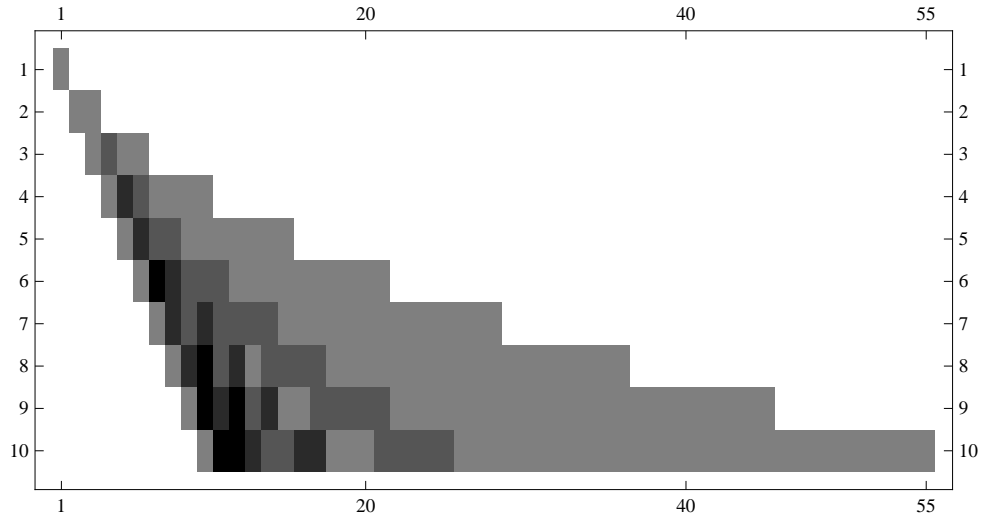
Fig. 4. Visualization of k . Black: k = 3 , light gray: k = 0 , white: out of range.
