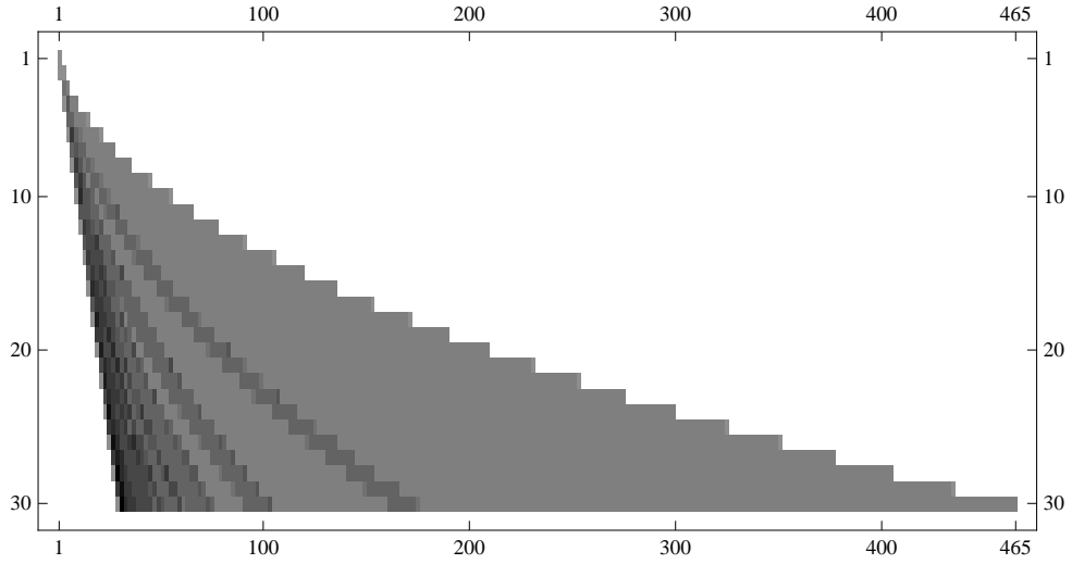
Fig. 5. Visualization of k . Black: k = 5 , light gray: k = 0 , white: out of range.
