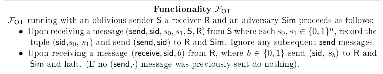
Figure 4: The Oblivious Transfer Functionality \mathcal{F}_{\text{OT}} .
