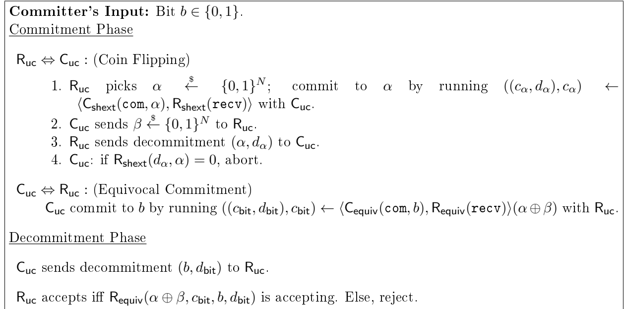
Figure 2: Computational UC Commitment Scheme (C_{uc}, R_{uc}) .
