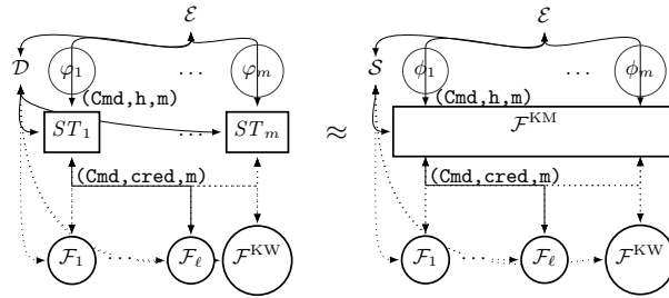
Fig. 1. Distributed security tokens in the network (left-hand side) and idealized functionality \mathcal{F}^{KM} in the same network (right-hand side), simplified.
