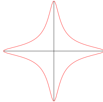
FIGURE 1. Edwards curve over \mathbb{R} .
