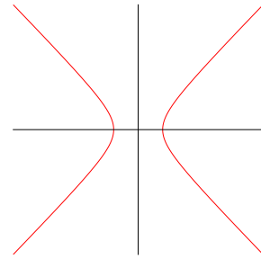
FIGURE 2. Projection of a Jacobi intersection curve over \mathbb{R} .
