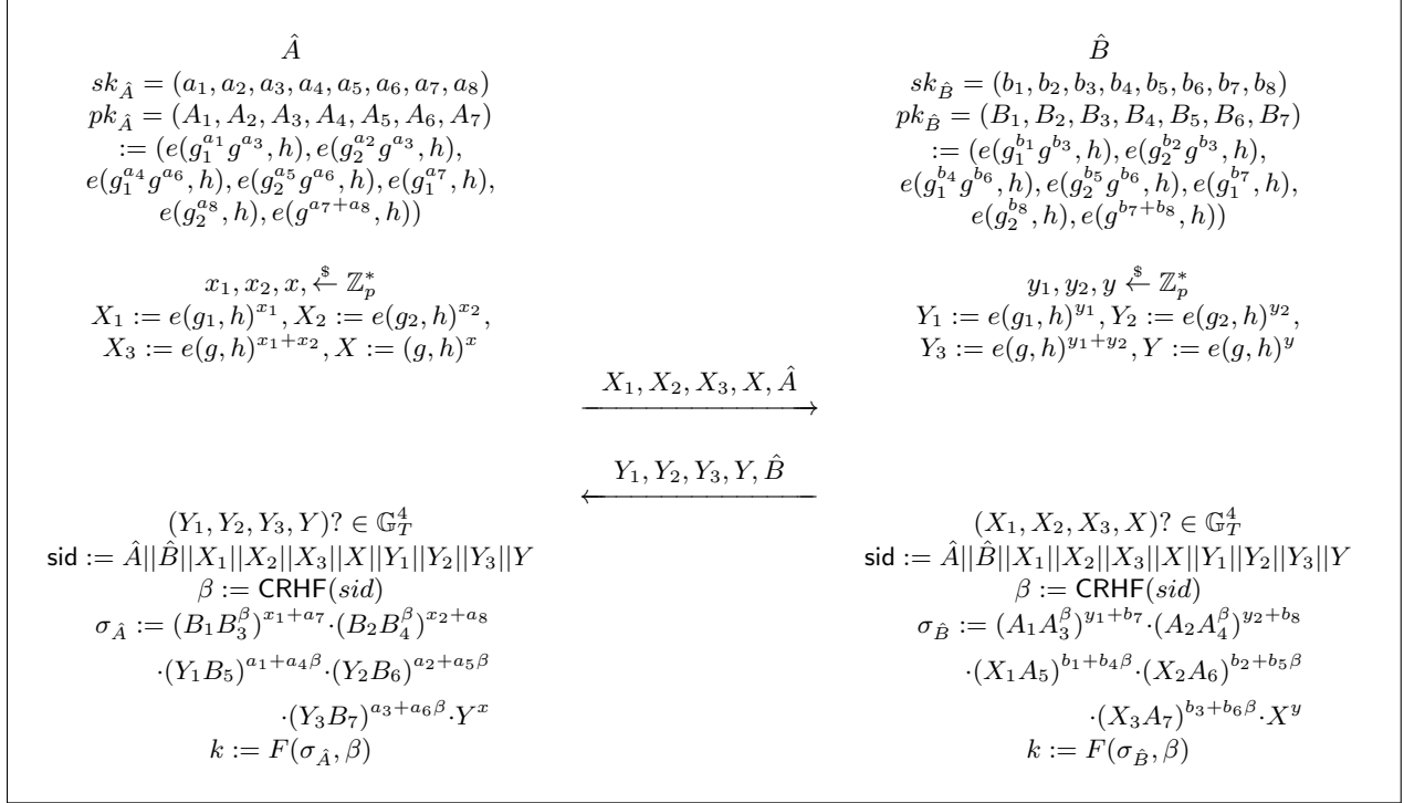
Figure 1: AKE Protocol from \pi\text{PRF}
