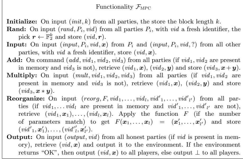
Fig. 4. The ideal functionality for MPC.
