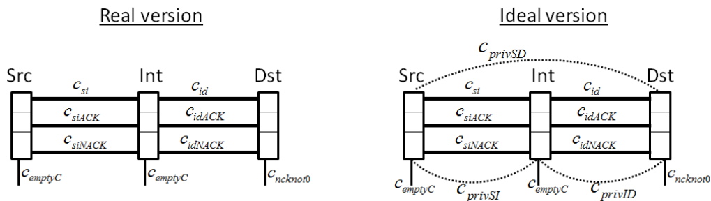
Figure 1: The difference between the real and ideal version of DTSN and SDTP.
