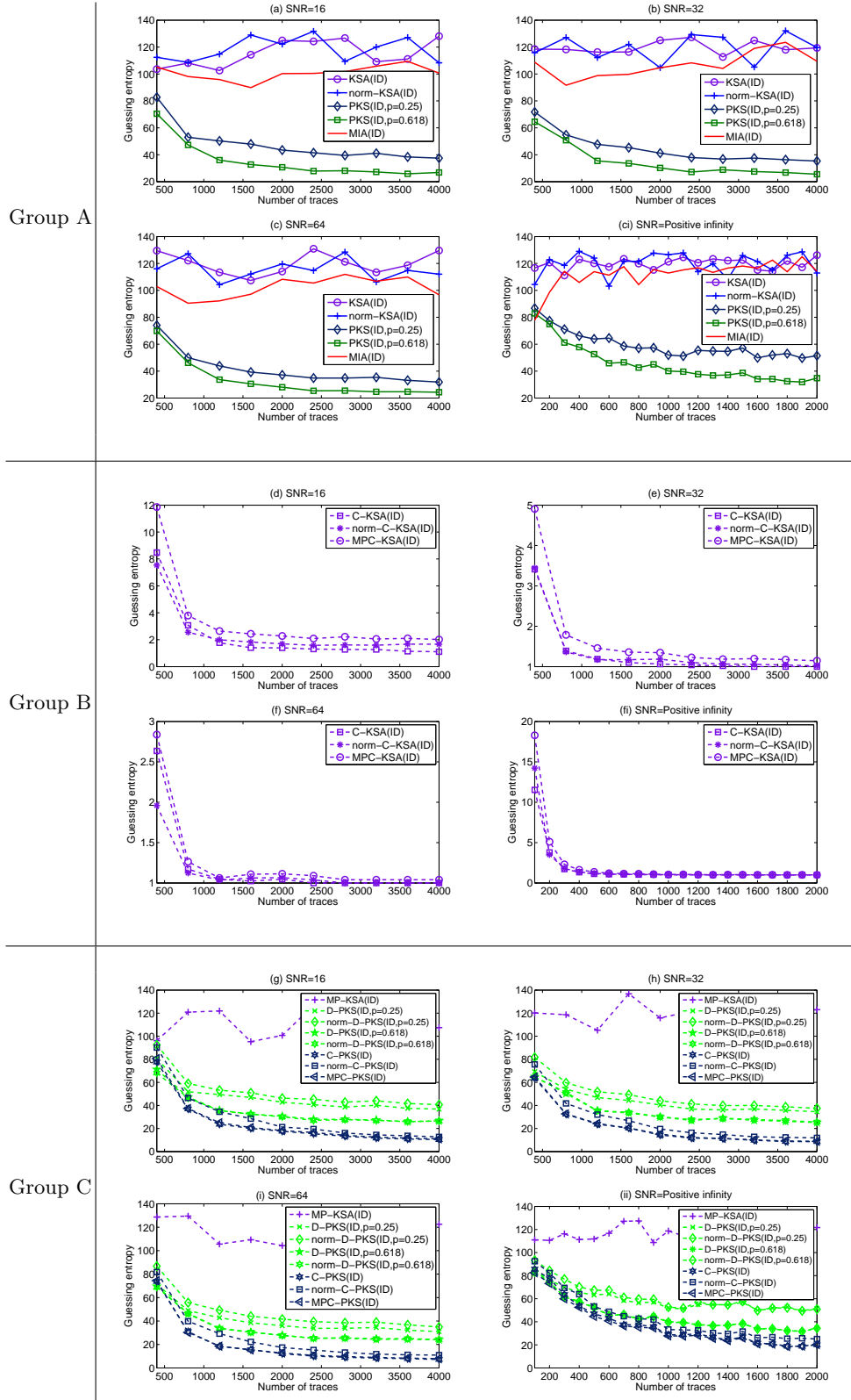
Fig. 13. Guessing entropy of different distinguishers against the first AES S-box in USWB leakage
