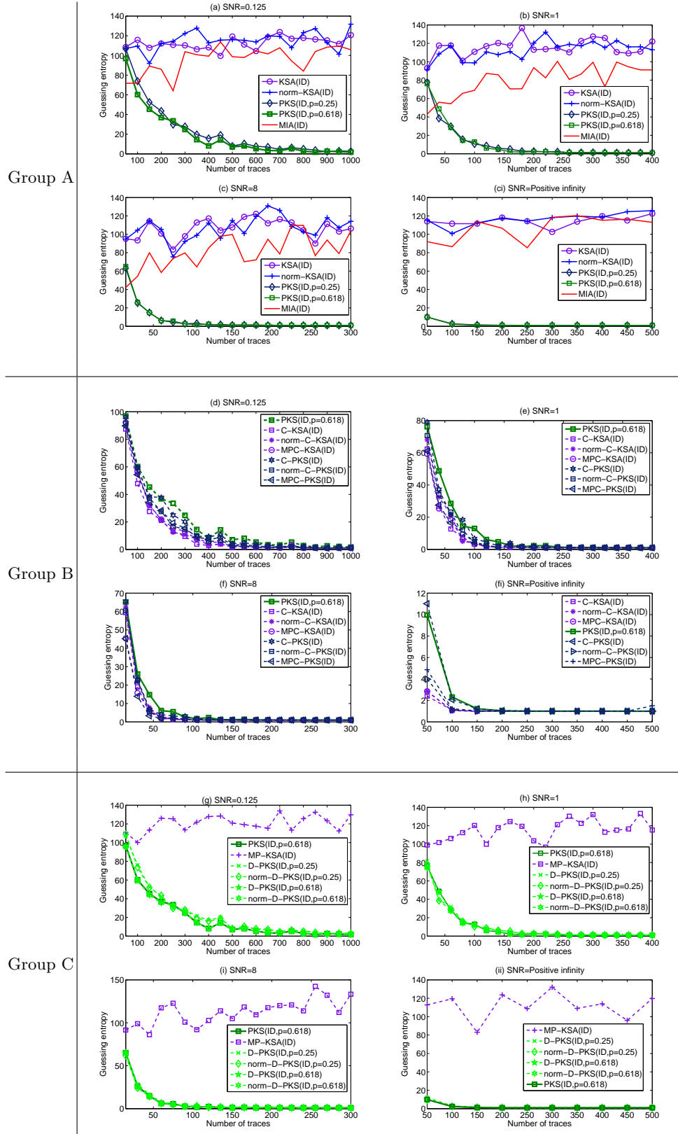
Fig. 11. Guessing entropy of different distinguishers against the first AES S-box in Hamming Weight leakage
