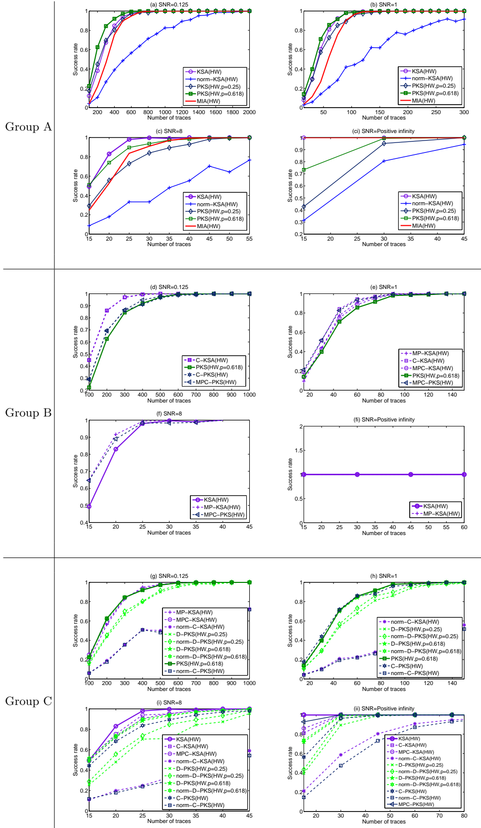
Fig. 3. Success rate of different distinguishers against the first AES S-box in Hamming Weight leakage
