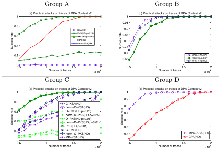
Fig. 8. Success rate for the KS test based distinguishers with HD model, MIA(HD) and CPA(HD) in attacks against the first AES S-box of the last round
