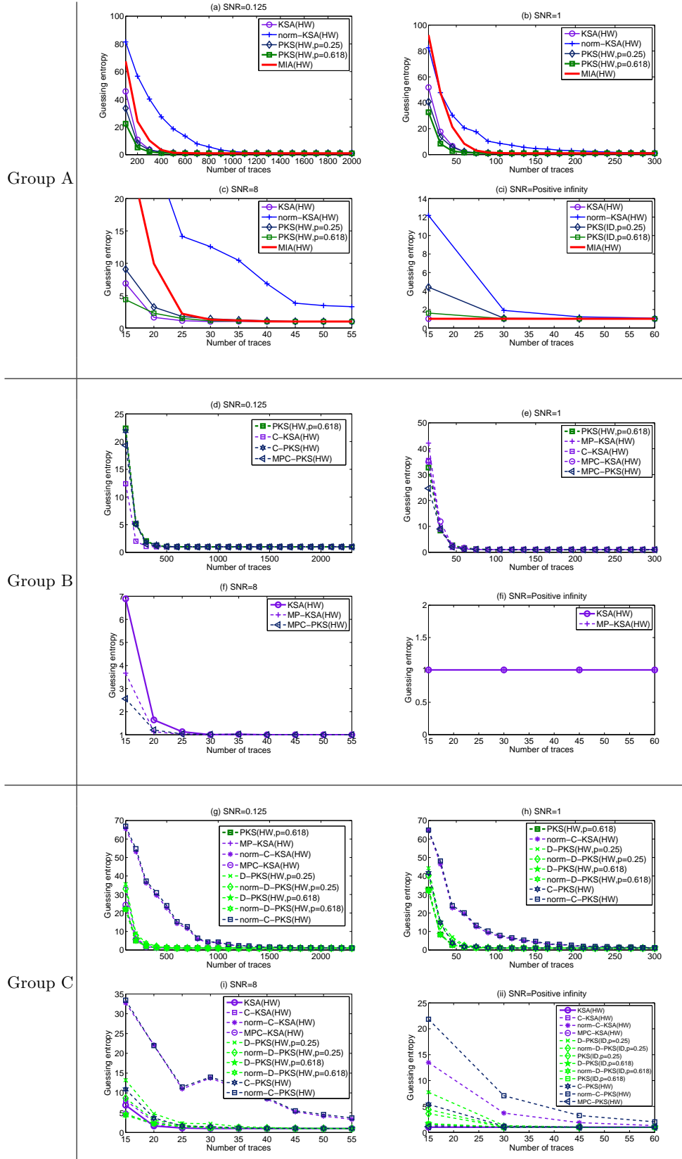
Fig. 10. Guessing entropy of different distinguishers against the first AES S-box in Hamming Weight leakage
