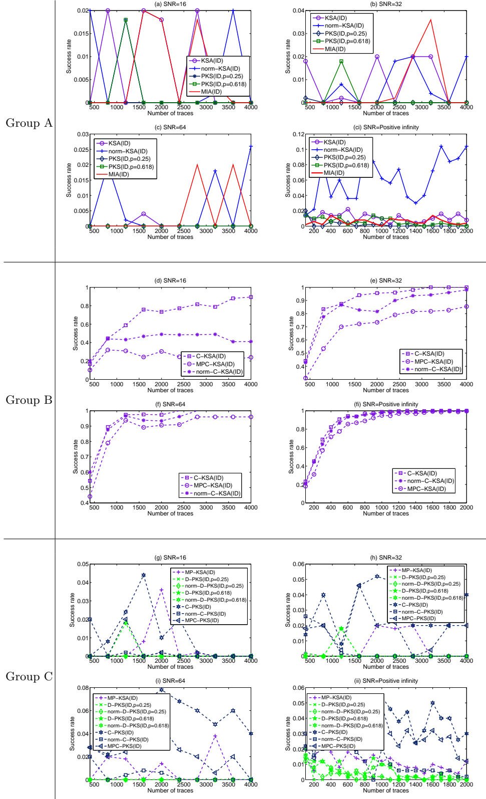
Fig. 6. Success rate of different distinguishers against the first AES S-box in USWB leakage
