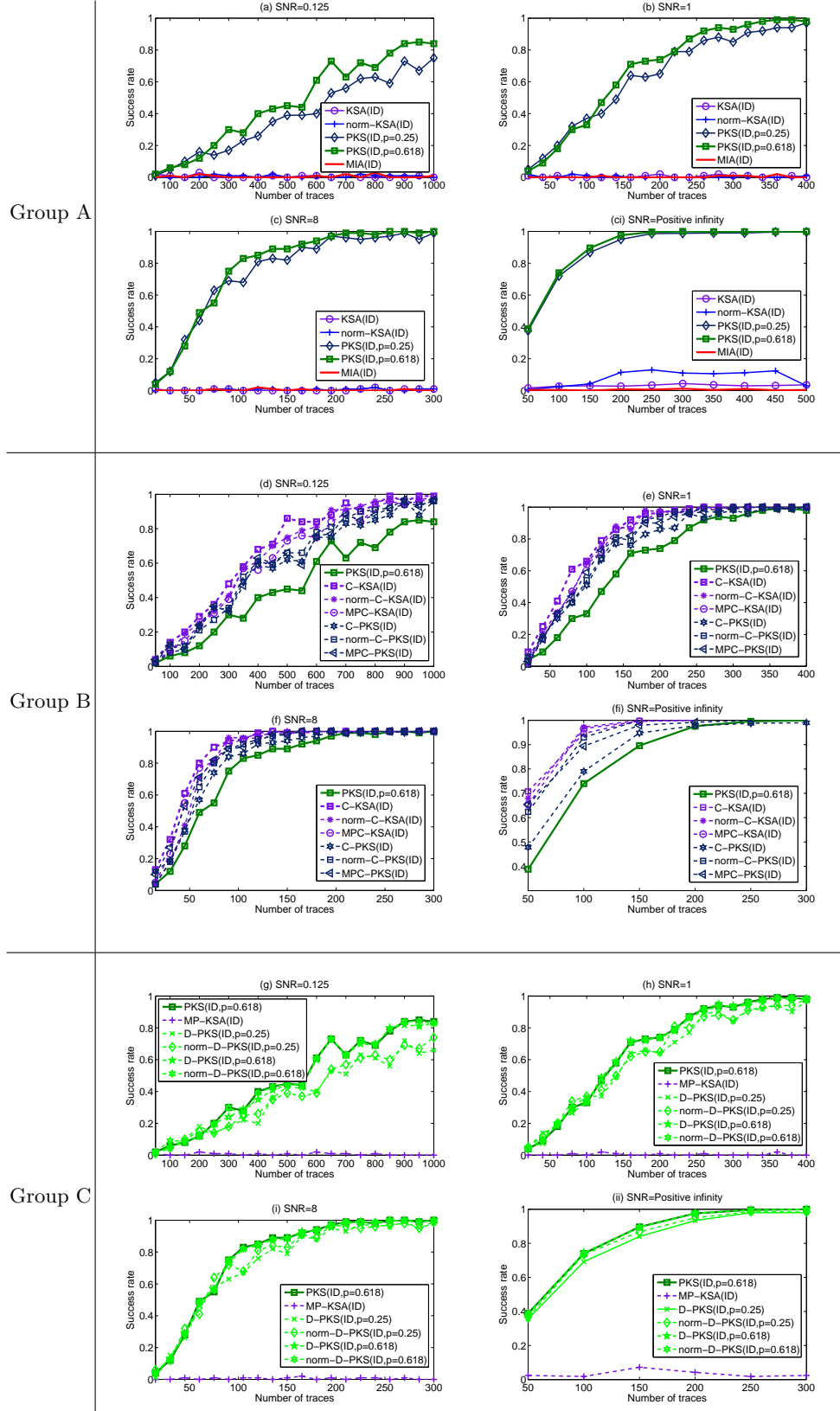
Fig. 4. Success rate of different distinguishers against the first AES S-box in Hamming Weight leakage
