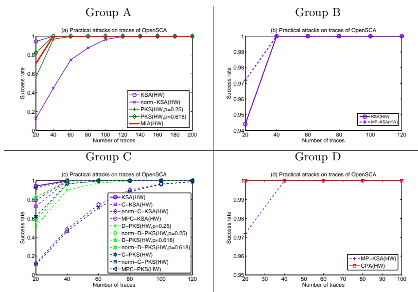
Fig. 7. Success rate for KS test based distinguishers with HW model, MIA(HW) and CPA(HW) in attacks against the first AES S-box
