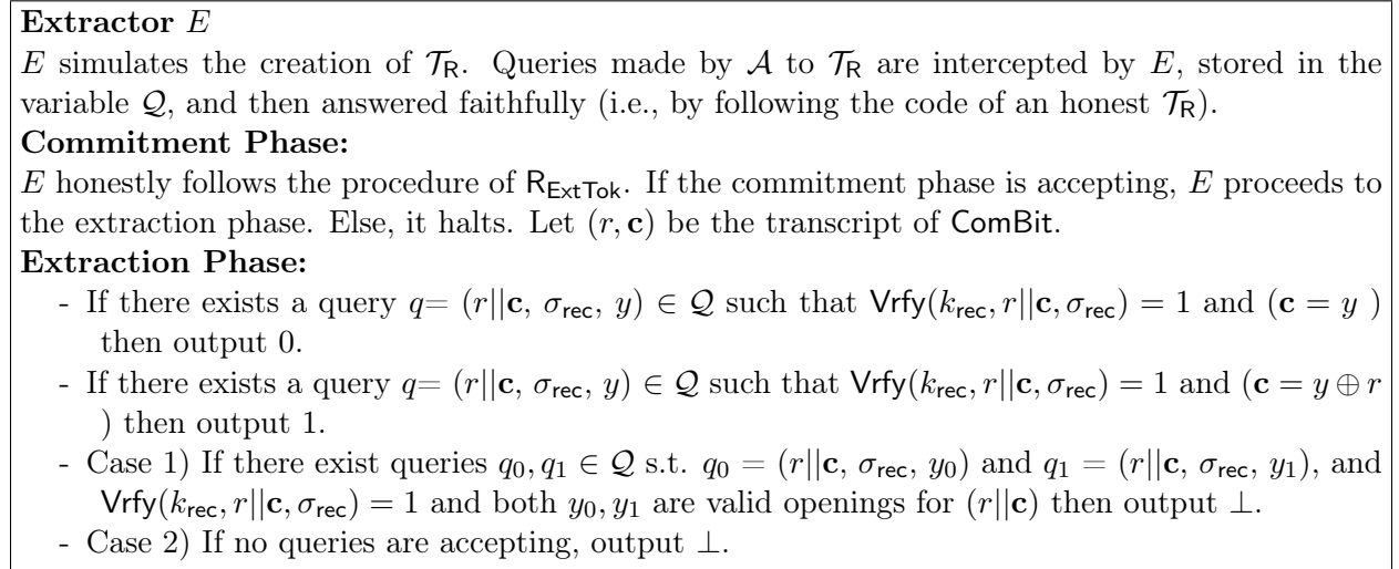
Figure 10: E : Extractor associated to ExtTok .
