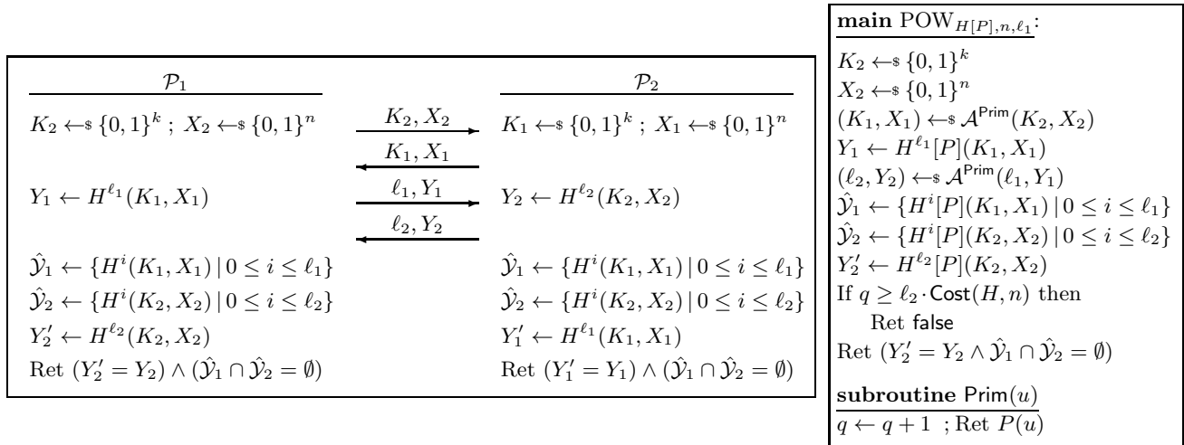
Figure 10: Example protocol ( left ) and adversarial \mathcal{P}_2 security game ( right ) for mutual proofs of work with keyed hash functions.
