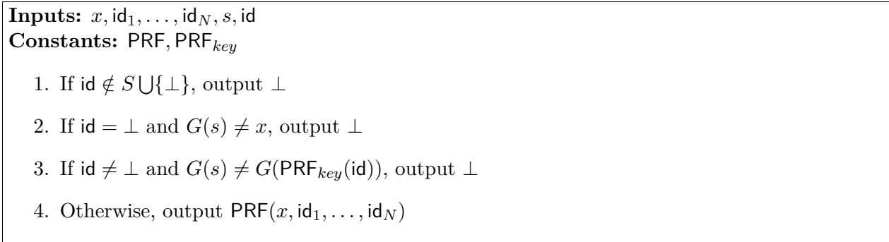
Figure 14: The program P_{IBBE} .
