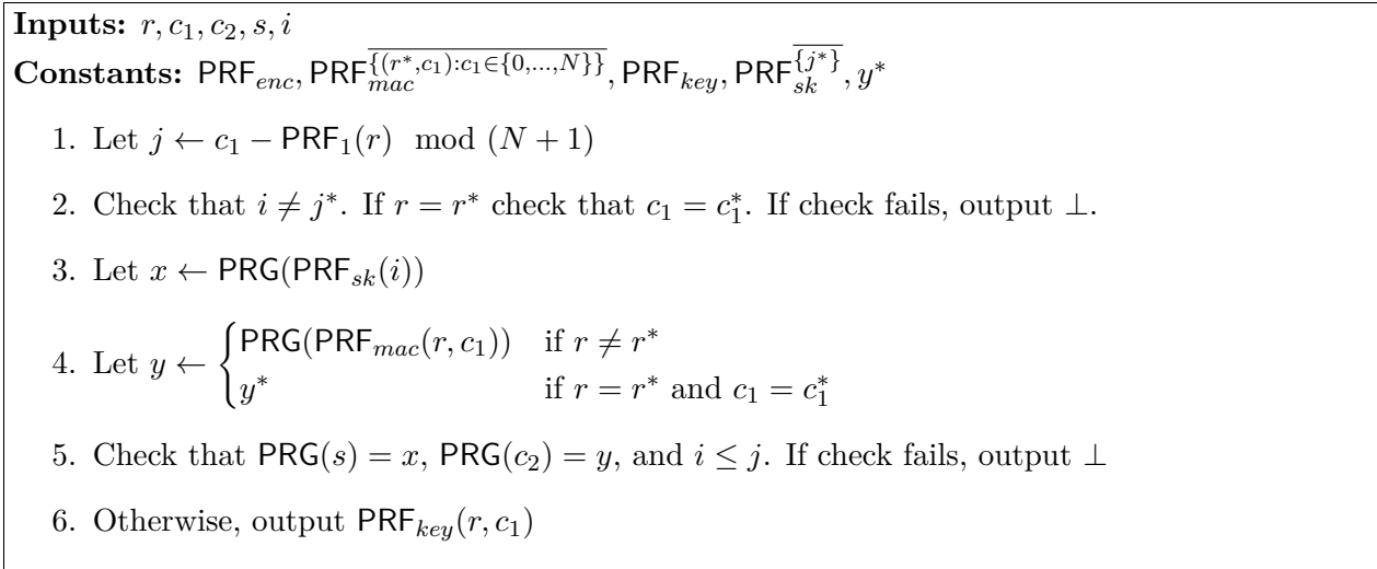
Figure 8: The program P'_{TT-Dec} .
