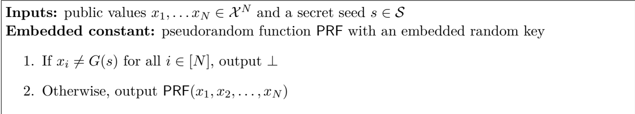
Figure 1: The program P_{KE} .
