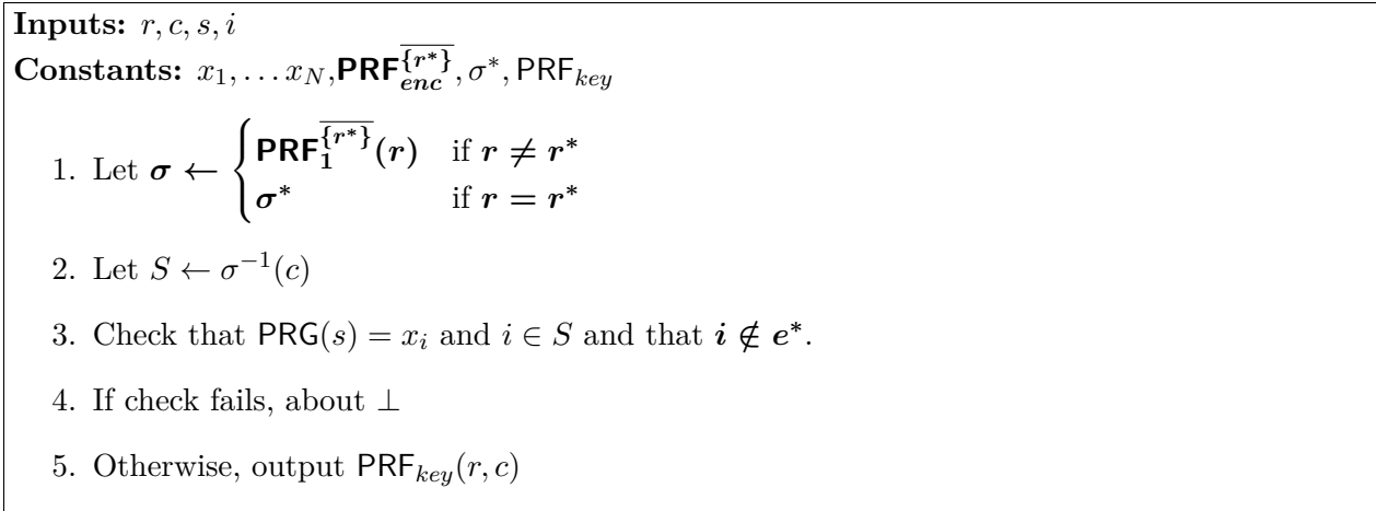
Figure 12: The program P'_{PBE-Dec} .
