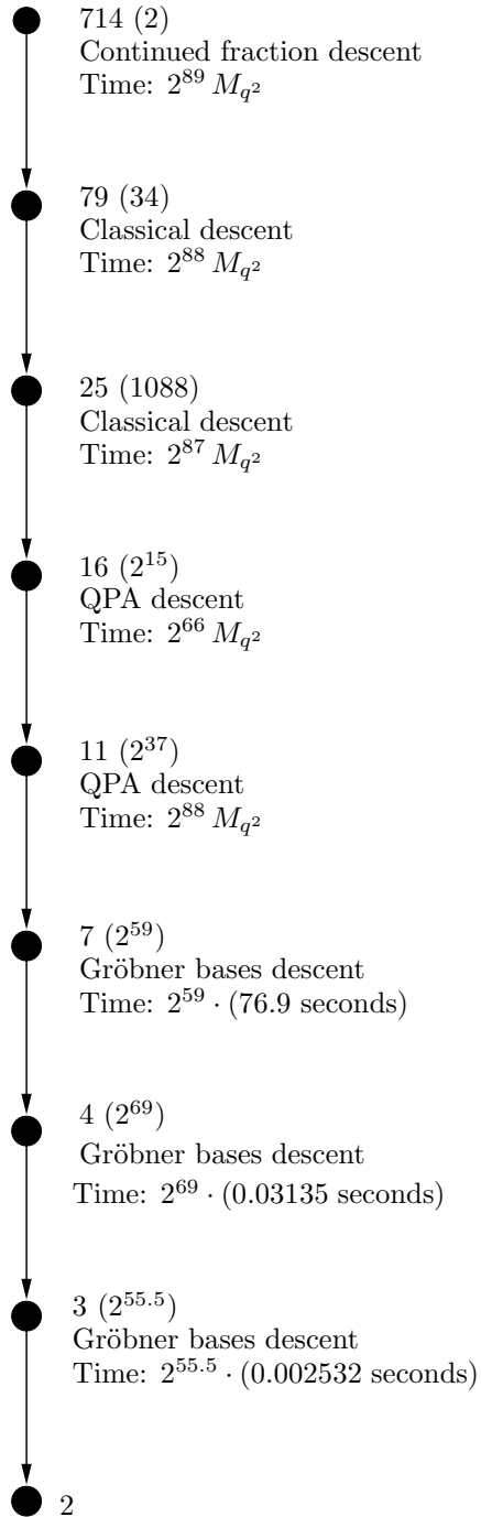
FIGURE 1. A typical path of the descent tree for computing an individual logarithm in \mathbb{F}_{3^{12 \cdot 1429}} ( q = 3^6 ). The numbers in parentheses next to each node are the expected number of nodes at that level. ‘Time’ is the expected time to generate all nodes at a level.
