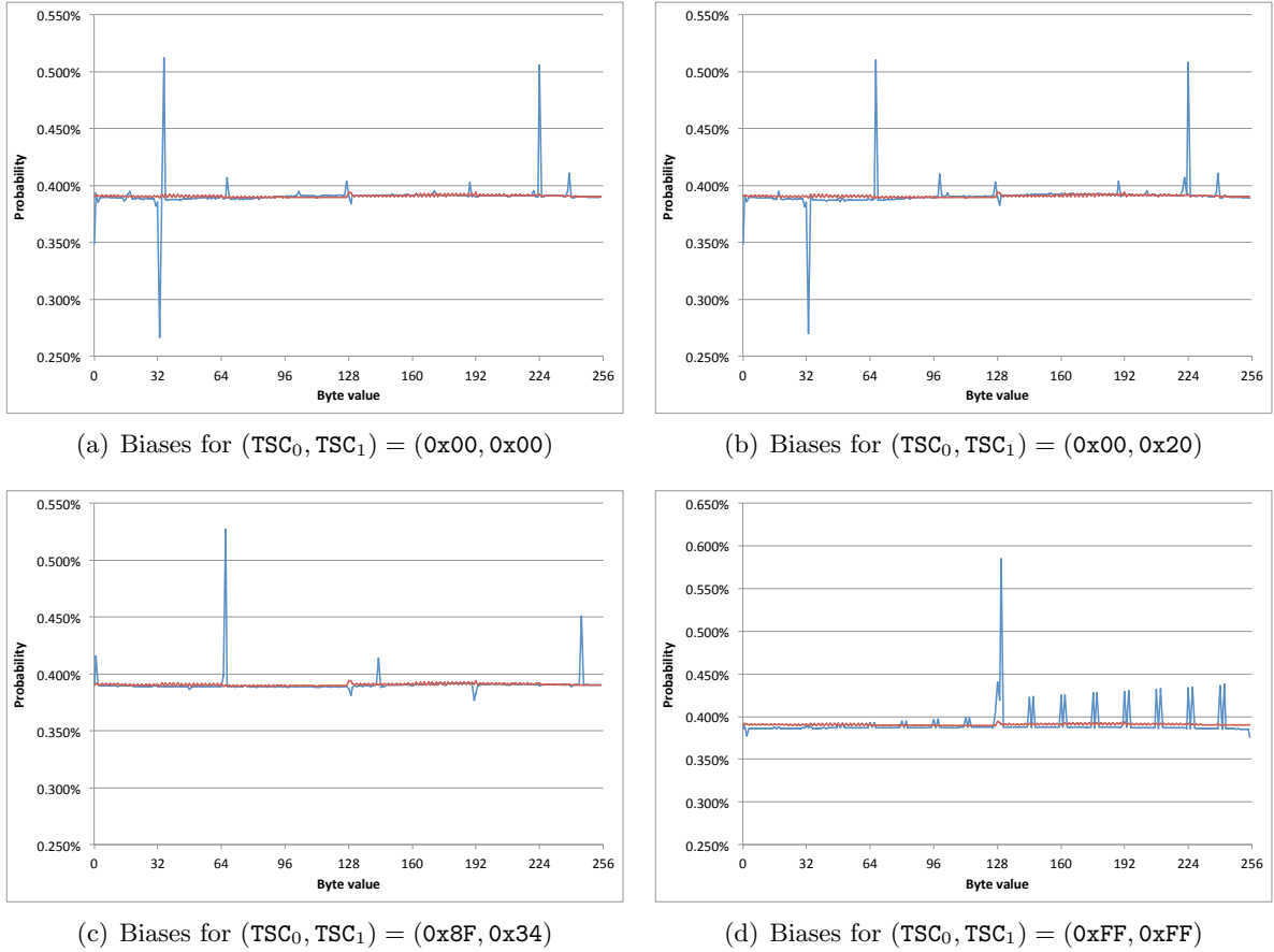
Figure 5: Measured distribution of the TKIP RC4 keystream at position Z_1 for (TSC_0, TSC_1) pairs (0x00, 0x00) , (0x00, 0x20) , (0x8F, 0x34) , (0xFF, 0xFF) (blue). These estimates were obtained by considering more than 2^{36} keys per (TSC_0, TSC_1) pair. For reference, we overlay the corresponding fully aggregated TKIP keystream biases (red).
