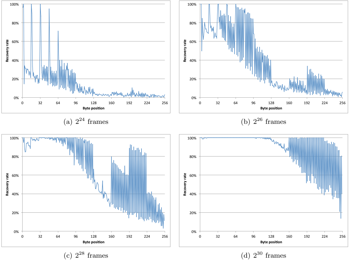
Figure 9: Success rate for 256 runs of attack based on fully aggregated TKIP biases using 2^{24} , 2^{26} , 2^{28} and 2^{30} simulated frames (4, 16, 64, and 256 keys generating 2^{22} frames each).
