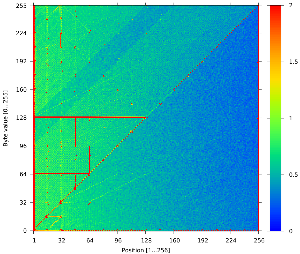
Figure 17: Pictorial representation of the correlation between position in TKIP keystream, byte value, and the corresponding strength of the largest occurring bias. The colouring scheme encodes the absolute difference between the occurring probabilities and the (expected) probability 1/256 , scaled up by a factor of 2^{16} , capped to a maximum of 2.
