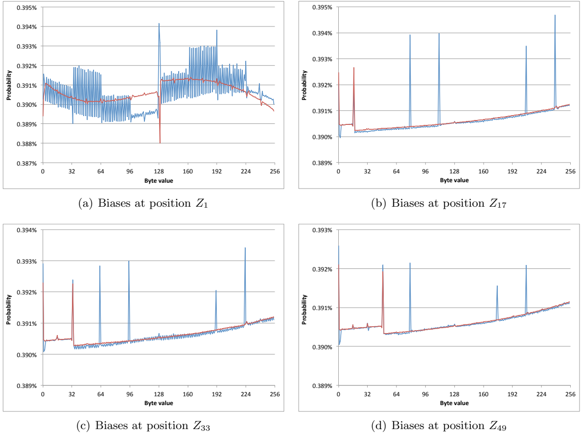
Figure 2: Measured distribution of the TKIP keystream at positions Z_1 , Z_{17} , Z_{33} , and Z_{49} (blue). These estimates were obtained by considering more than 2^{41} KM-generated keys. For reference, we overlay the biases of the RC4 keystream with random 128-bit keys (red).
