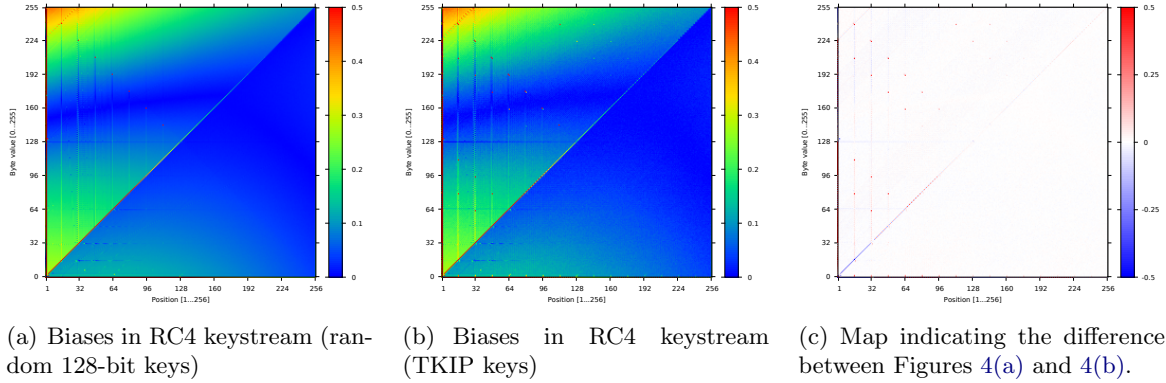
Figure 4: Pictorial representation of biases in RC4 keystreams for random 128-bit keys and for TKIP keys, for different positions (x-axis) and byte values (y-axis). For each position we encode the bias in the keystream for the (position,value) combination as a colour; in Figures 4(a) and 4(b) the colouring scheme encodes the absolute biases, i.e., the absolute difference between the occurring probabilities and the (expected) probability 1/256 , scaled up by a factor of 2^{16} , capped to a maximum of 0.5. In Figure 4(c), the colour encodes the difference between the absolute biases arising for random 128-bit keys and for TKIP keys, scaled up by a factor of 2^{16} and capped to the range [-0.5, 0.5] . We provide high-resolution versions of Figures 4(a)–4(c) on pages 22–24.
