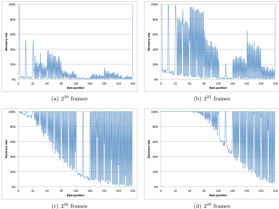
Figure 11: Success rate for attack on TKIP based on aggregation of TSC_0 values for 256 simulations, each using 2^{20} , 2^{22} , 2^{26} , and 2^{28} frames. See Figure 10(c) for the success rate for 2^{24} frames.
