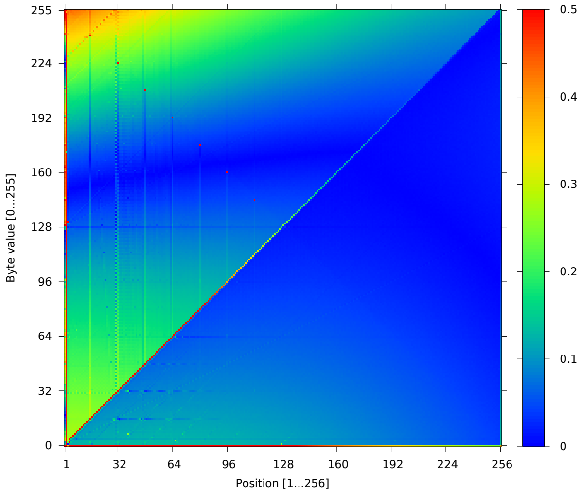
Figure 13: Pictorial representation of biases in RC4 keystreams for random 128-bit keys, for different positions (x-axis) and byte values (y-axis). For each position we encode the bias in the keystream for the (position,value) combination as a colour; the colouring scheme encodes the absolute biases, i.e., the absolute difference between the occurring probabilities and the (expected) probability 1/256 , scaled up by a factor of 2^{16} , capped to a maximum of 0.5.
