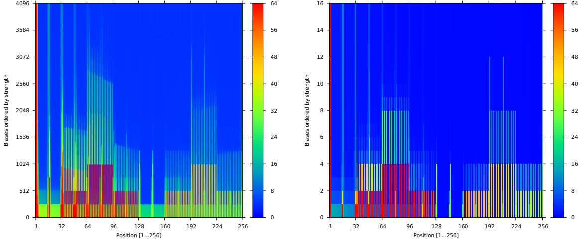
(a) Largest 4096 biases of the RC4 keystream, taken over all 2^{16} ( \text{TSC}_0, \text{TSC}_1 ) combinations
