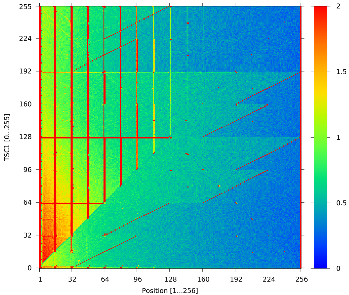
Figure 16: Pictorial representation of the correlation between position in TKIP keystream, TSC_1 value, and the corresponding strength of the largest occurring bias. The colouring scheme encodes the absolute difference between the occurring probabilities and the (expected) probability 1/256 , scaled up by a factor of 2^{16} , capped to a maximum of 2.
