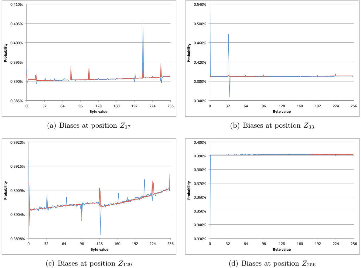
Figure 6: Measured distribution of the TKIP keystream at positions Z_{17} , Z_{33} , Z_{129} , Z_{256} for (TSC_0, TSC_1) pair (0x00, 0x00) (blue; see Figure 5(a) for distribution of Z_1 ). These estimates were obtained by considering more than 2^{36} keys per TSC pair. For reference, we overlay the corresponding fully aggregated TKIP keystream biases (red).
