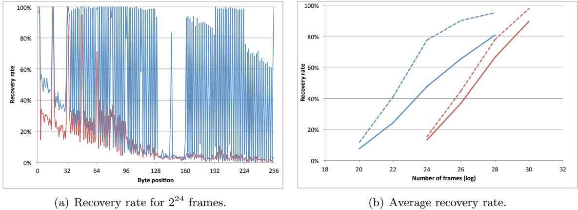
Figure 12: Comparison of attack using fully aggregated biases (red) and attack based on aggregation over all TSC_0 values (blue). Figure (a) shows the recovery rates of the two attacks for 256 runs each with 2^{24} simulated frames. Figure (b) shows the average recovery rates of the two attacks. The dashed lines correspond to the average recovery rates for even positions.
