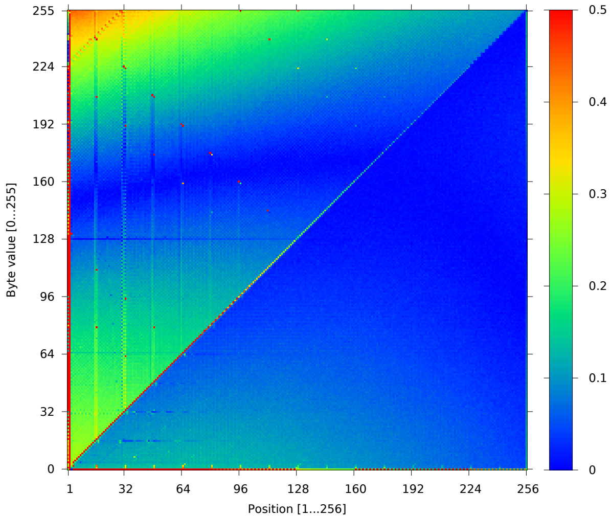
Figure 14: Pictorial representation of biases in RC4 keystreams for TKIP keys, for different positions (x-axis) and byte values (y-axis). For each position we encode the bias in the keystream for the (position,value) combination as a colour; the colouring scheme encodes the absolute biases, i.e., the absolute difference between the occurring probabilities and the (expected) probability 1/256 , scaled up by a factor of 2^{16} , capped to a maximum of 0.5.
