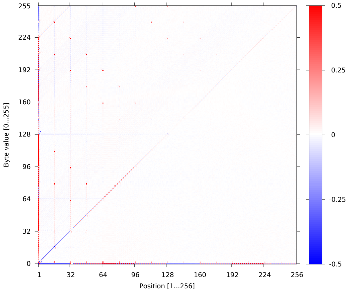
Figure 15: Pictorial representation of the difference of biases in RC4 keystreams for random keys and TKIP keys, for different positions (x-axis) and byte values (y-axis). At each point we encode as a colour the difference between the absolute biases arising for random 128-bit keys and for TKIP keys for the specific (position,value) combination, scaled up by a factor of 2^{16} and capped to the range [-0.5, 0.5]
