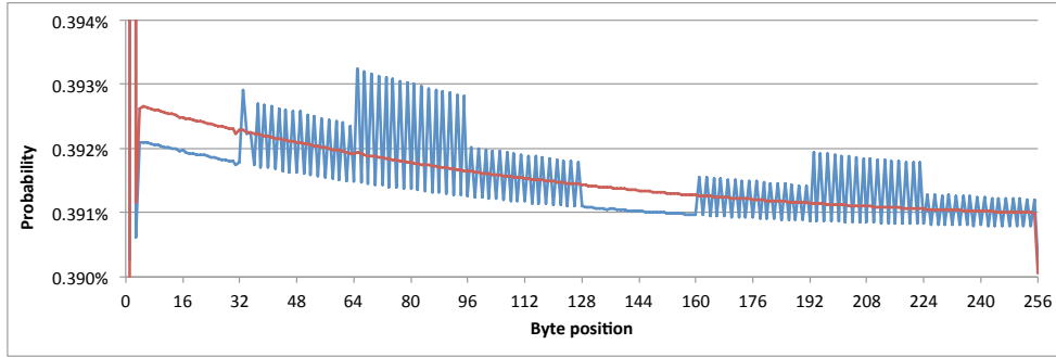
Figure 3: Strength of the bias towards 0x00 of TKIP keystream bytes at positions 1–256 (blue). The red line corresponds to the biases of RC4 with random 128-bit keys.
