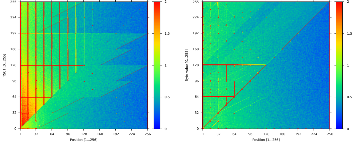
(a) Strength of largest available bias for each combination of position and \text{TSC}_1 value
