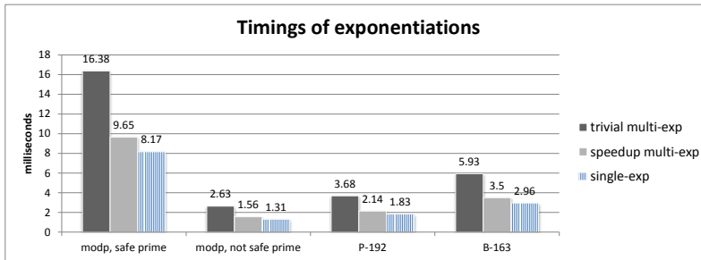
Fig. 7. Average timings of trivial and speedup computation of exponentiations, taken over 10000 executions, over various base groups. Experiment is done over a laptop (Intel 2.0GHz CPU, 8GB RAM) running Ubuntu 12.04 LTS. The C compiler is g++ 4.6.3 using NTL 6.0.0 and GMP 5.1.1 libraries.
