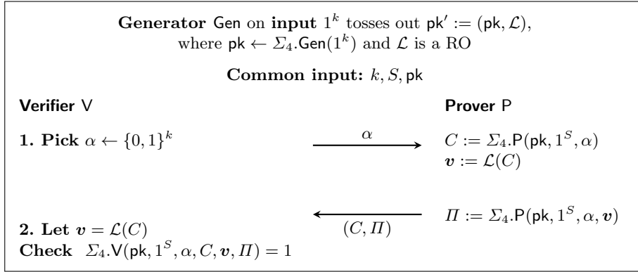
Fig. E.1. The 2-messages PoSpace protocol \Sigma_2 = (\text{Gen}, \text{P}, \text{V}) .
