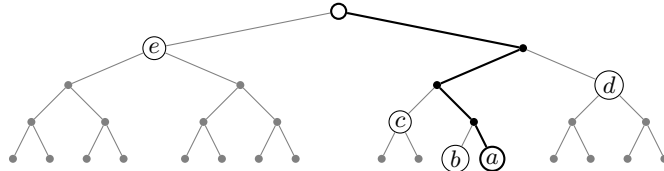
Fig. F.1. An example of opening: \mathbf{c} = (a, b, c, d, e)
