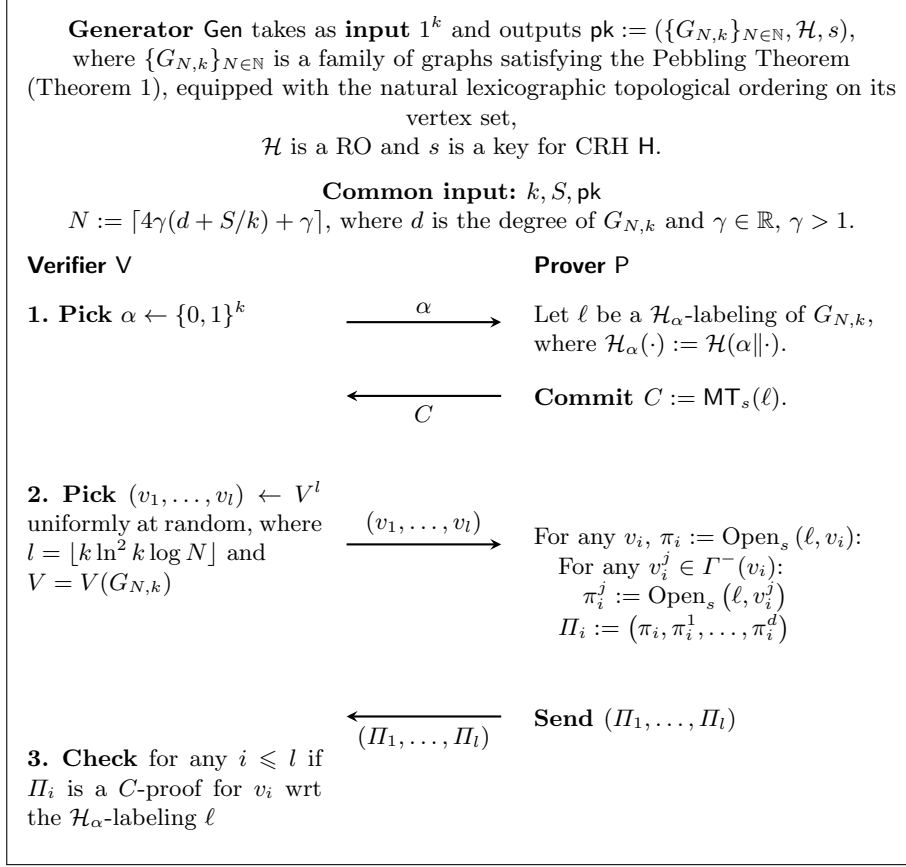
Fig. 3.1. The 4-message PoSpace protocol \Sigma_4 .
