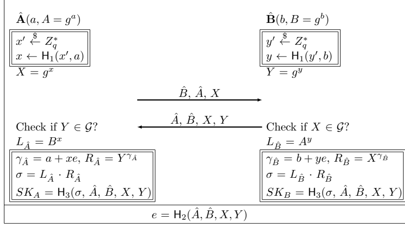
Figure 2: The description of the VOAKE protocol.
