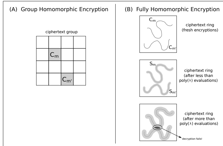
Fig. 1. Differences between group homomorphic encryption and FHE: (A) shows that each C_m is a coset of \mathcal{C}_1 in \mathcal{C} (Fact 1), while the decryption is a group homomorphism; (B) shows first that C_m and C_{m'} are subsets and not necessarily cosets in \mathcal{C} , second that the decryption runs correctly on \text{poly}(\lambda) evaluations of ciphertexts, and third that the decryption might fail if exponentially many evaluations have been performed, meaning that the decryption is not necessarily group homomorphic.
