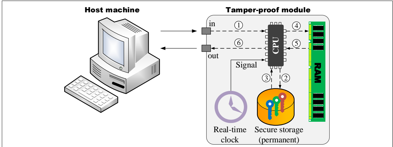
Figure 2. A TPM consists of input/output ports, a CPU, an RTC, a RAM, and a secure permanent storage. The CPU reads information from the input port (1), addresses the secure storage (2), retrieves the relevant key (3), communicates with the RAM (4 & 5), and writes information to the output port (6). The real-time clock signals the CPU every \tau seconds, upon which the CPU updates every key in the database.
