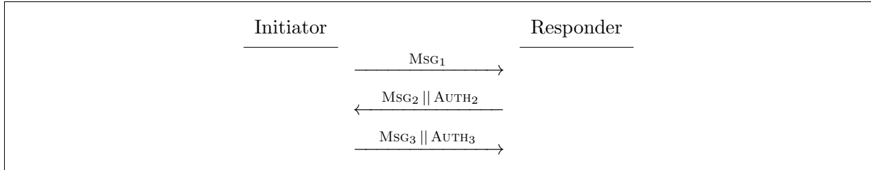
Protocol 1. The proposed AKE protocol. Details are described in Section 3 .
