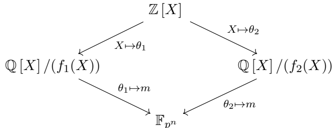
Figure 1: Commutative diagram of NFS.
