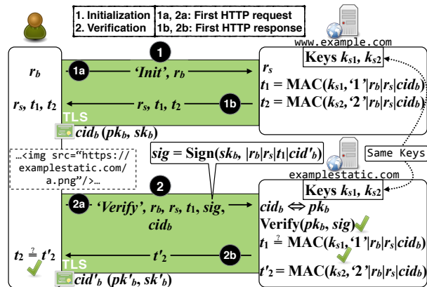
Figure 10: SISCA adapted for cross-origin communication (the origins share the same SISCA keys), when the browser uses a different Channel ID for each origin. Here, www.example.com performs a cross-origin request to examplestatic.com .
