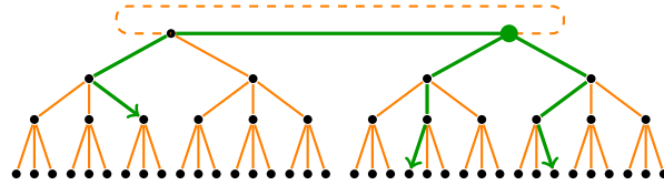
Fig. 4. Three non-backtracking paths suffice to reach a given level.
