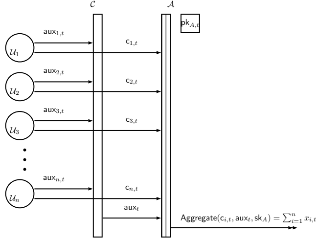
Fig. 1. Overview of our protocol for a single time interval t . \text{pk}_{\mathcal{A},t} is public known value.
