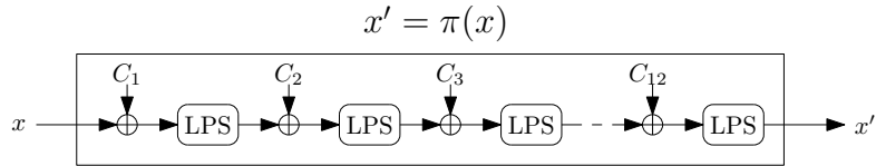
Figure 5: The 512-bit permutation \pi used by STRIBOB.
