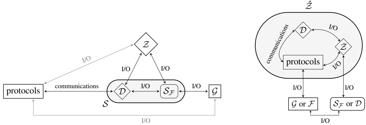
(a) The simulator \mathcal{S} interacting with the protocol \pi and the global functionality \mathcal{G} .
