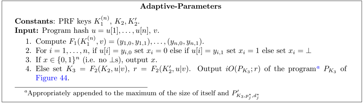
Figure 43: Program Adaptive-Parameters
